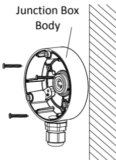
Figure 2-5 Secure the Junction Box on the Wall/Ceiling
