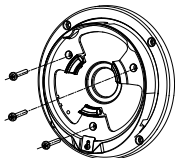
Figure 2-13 Secure Screws on Junction Box's Cover
