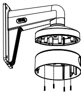
Figure 2-21 Attach the Back Box/Base Plate to the Bracket
